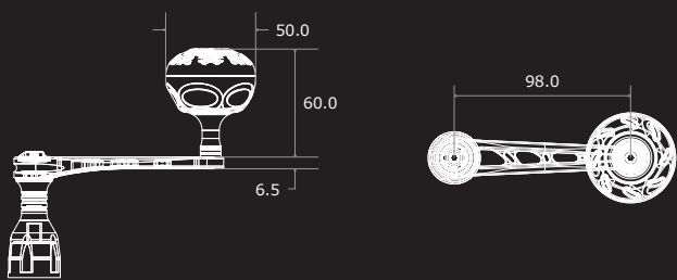
POWER 98 Dimensions (unit: mm)
