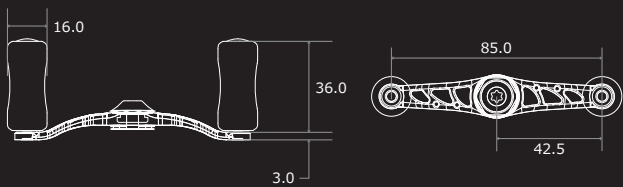
CRANK 85 Dimensions (unit: mm)
