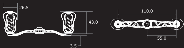
CRANK Feather 110 Dimensions (unit: mm)
