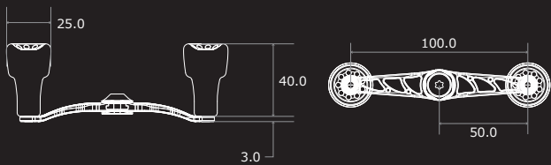
CRANK 100 Dimensions (unit: mm)
