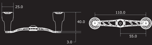
CRANK 110 Dimensions (unit: mm)
