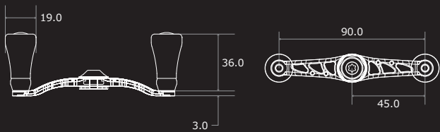
CRANK 90 Dimensions (unit: mm)
