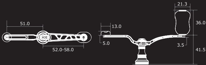
UNION 52-58 Dimensions (unit: mm)
