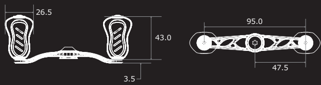
CRANK Feather 95 Dimensions (unit: mm)
