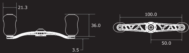
CRANK Feather 100 Dimensions (unit: mm)
