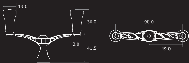
WING 98 Dimensions (unit: mm)
