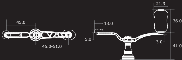
UNION 45-51 Dimensions (unit: mm)
