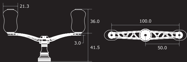
WING 100 Dimensions (unit: mm)
