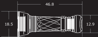
Custom Balancer Dimensions (unit:mm)
