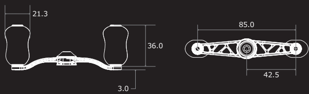
CRANK Feather 85 Dimensions (unit: mm)
