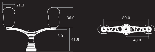
WING 80 Dimensions (unit: mm)
