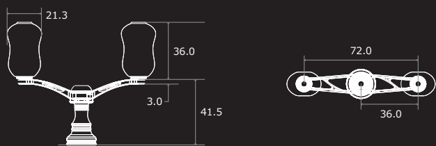
WING 72 Dimensions (unit: mm)
