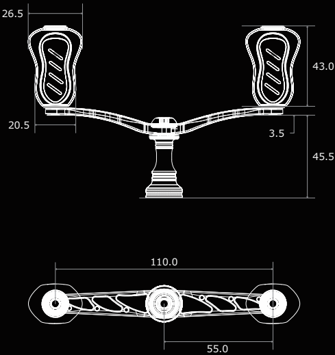
WING 110 Dimensions (unit: mm)
