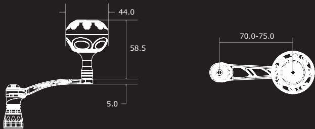
POWER 70-75 Dimensions (unit: mm)
