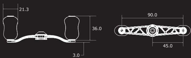
CRANK Feather 90 Dimensions (unit: mm)
