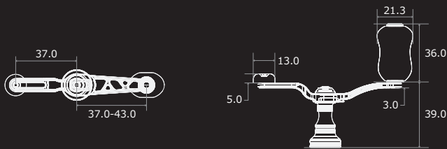
UNION 37-43 Dimensions (unit: mm)
