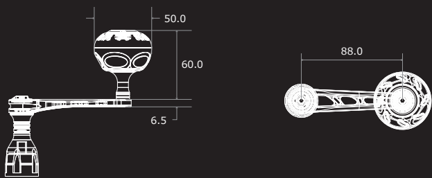
POWER 88 Dimensions (unit: mm)
