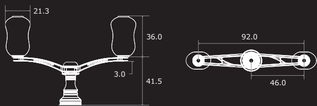
WING 92 Dimensions (unit: mm)
