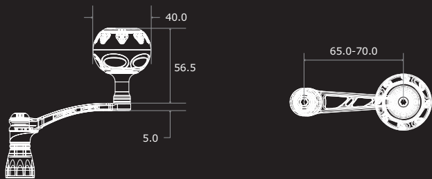
POWER 65-70 Dimensions (unit: mm)
