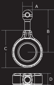
Q.R.A Dimensions (unit: mm)
